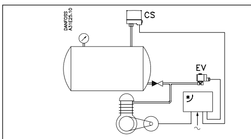
Example 3 Control of an air compressor with a CS. An EVI 3 solenoid valve is recommended where there is need for especially fast pressure relief.
