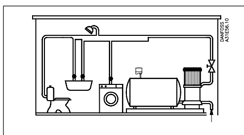
Example 5 Pressure boosting system for domestic circuits. A type CS switch is used to start/stop the pump.
