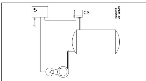
Example 4 Control of a centrifugal pump with a CS, via an automatic star-delta switch, motor starter, or similar.
