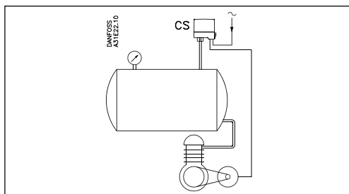
Example 1 Control of an air compressor with a CS pressure switch.
