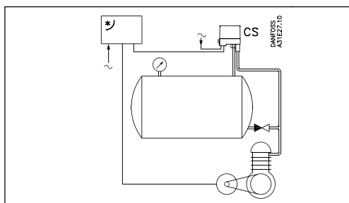
Example 2 Control of a compressor with a CS pressure switch fitted with pressure relief valve. Note the check valve between pressure relief line and reservoir.
