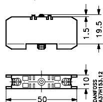
Auxiliary contact block CB
