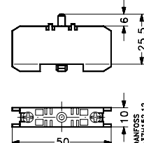
Start contact block CB-S
