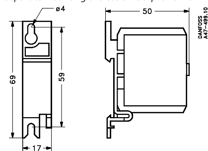
Separate mounting of electronic clip-on timer ETB
