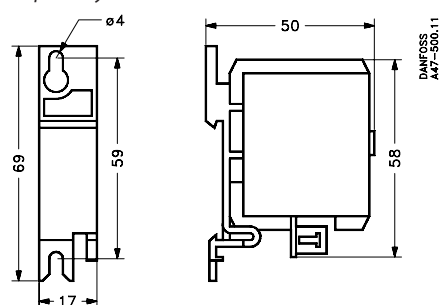
RC Element for contactors CI 6, 9, 12, 15, 16, 20, 25, 30
