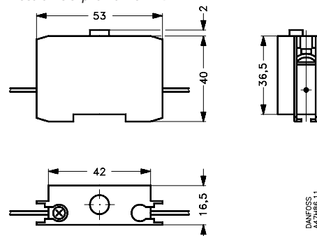
Electronic clip-on timer ETB
